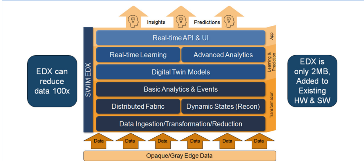
Figure 1: SWIM overview
